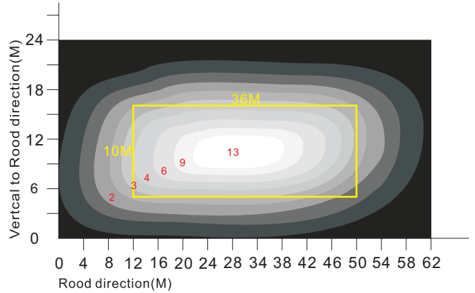
Lamp height:12M The effective lumination area can be realized just as the yellow rectangular area indicated ,36M*10M. Average lumination: 8Lux. Road surface evenness ratio:68%
