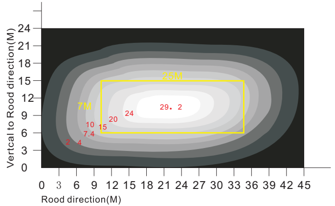
Lamp height:8M The effective lumination area can be realized just as the yellow rectangular area indicated ,25M*7M. Average lumination: 22Lux. Road surface evenness ratio:68%
