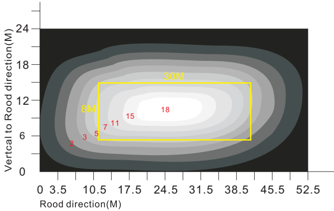
Lamp height:10M The effective lumination area can be realized just as the yellow rectangular area indicated ,30M*8M. Average lumination: 13Lux. Road surface evenness ratio:68%
