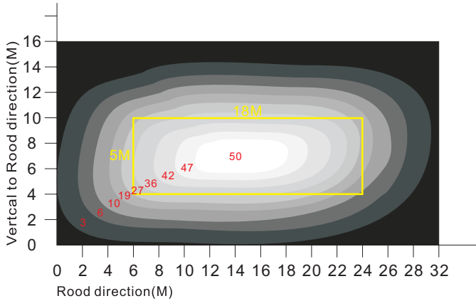
Lamp height:6M The effective lumination area can be realized just as the yellow rectangular area indicated ,18M*5M. Average lumination: 43Lux. Road surface evenness ratio:68%
